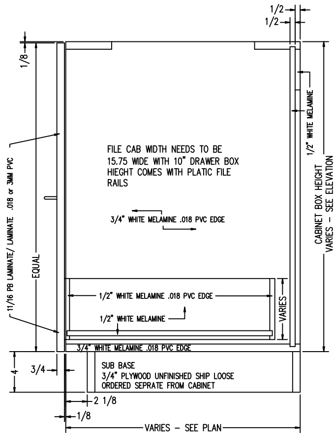
TYPICAL BOD1D FOR SUB BASE SCALE: 1-1/2" = 1'-0"
