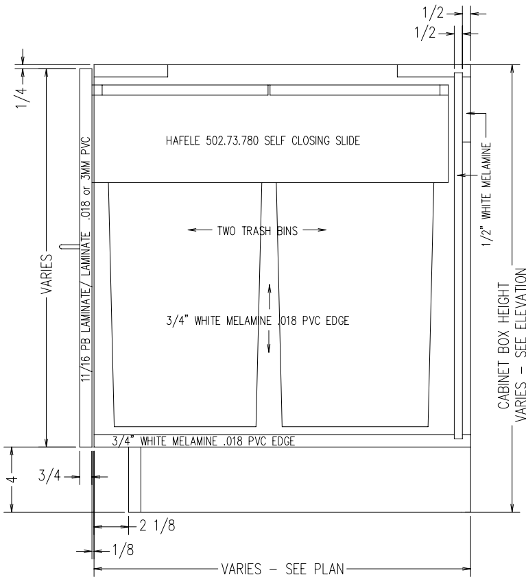
TYPICAL B0D1D-TRASH INTEGRAL TOE KICK
