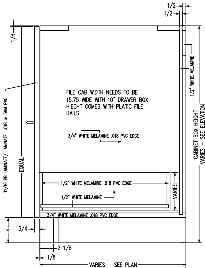
TYPICAL BOD1D INTEGRAL TOE KICK SCALE: 1-1/2" = 1'-0"
