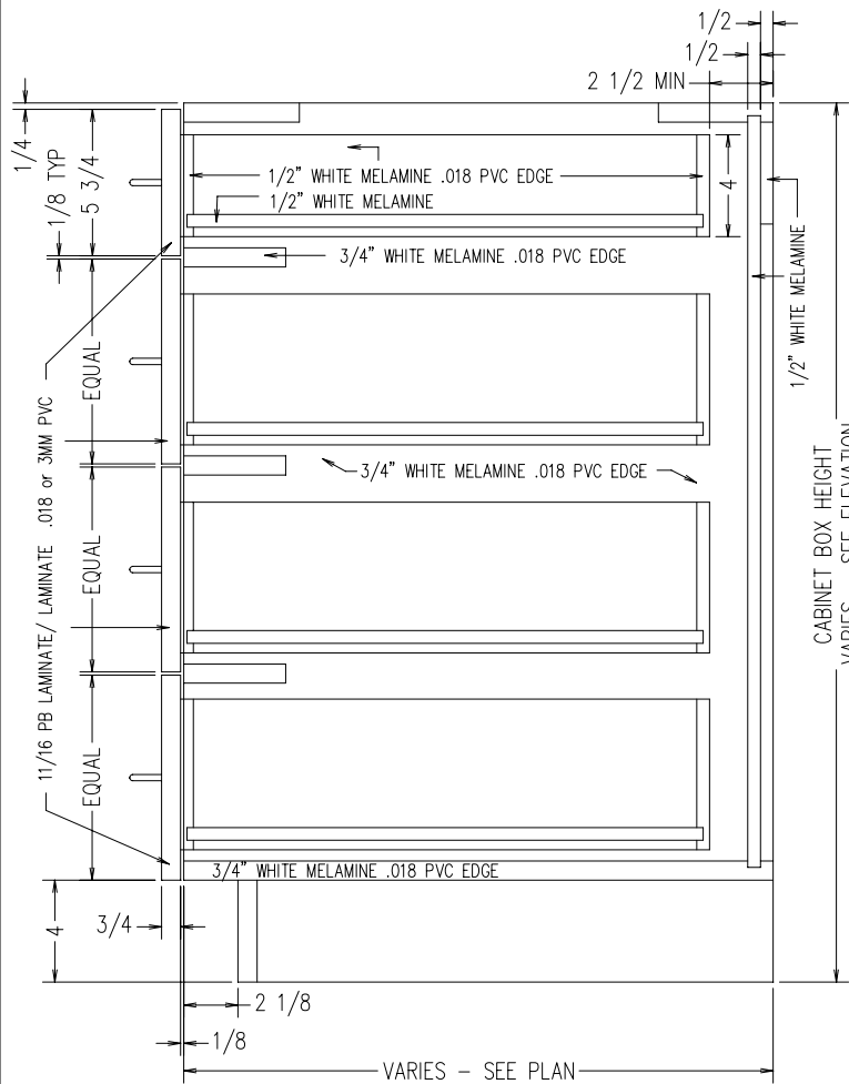
TYPICAL B0D4D INTEGRAL TOE KICK SCALE: 1-1/2" = 1'-0"
