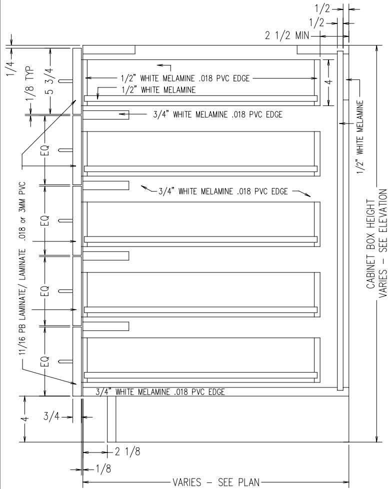
TYPICAL B0D5D INTEGRAL TOE KICK SCALE: 1-1/2" = 1'-0"
