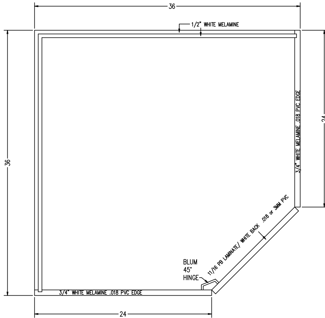
TYPICAL B1D-CORNER
