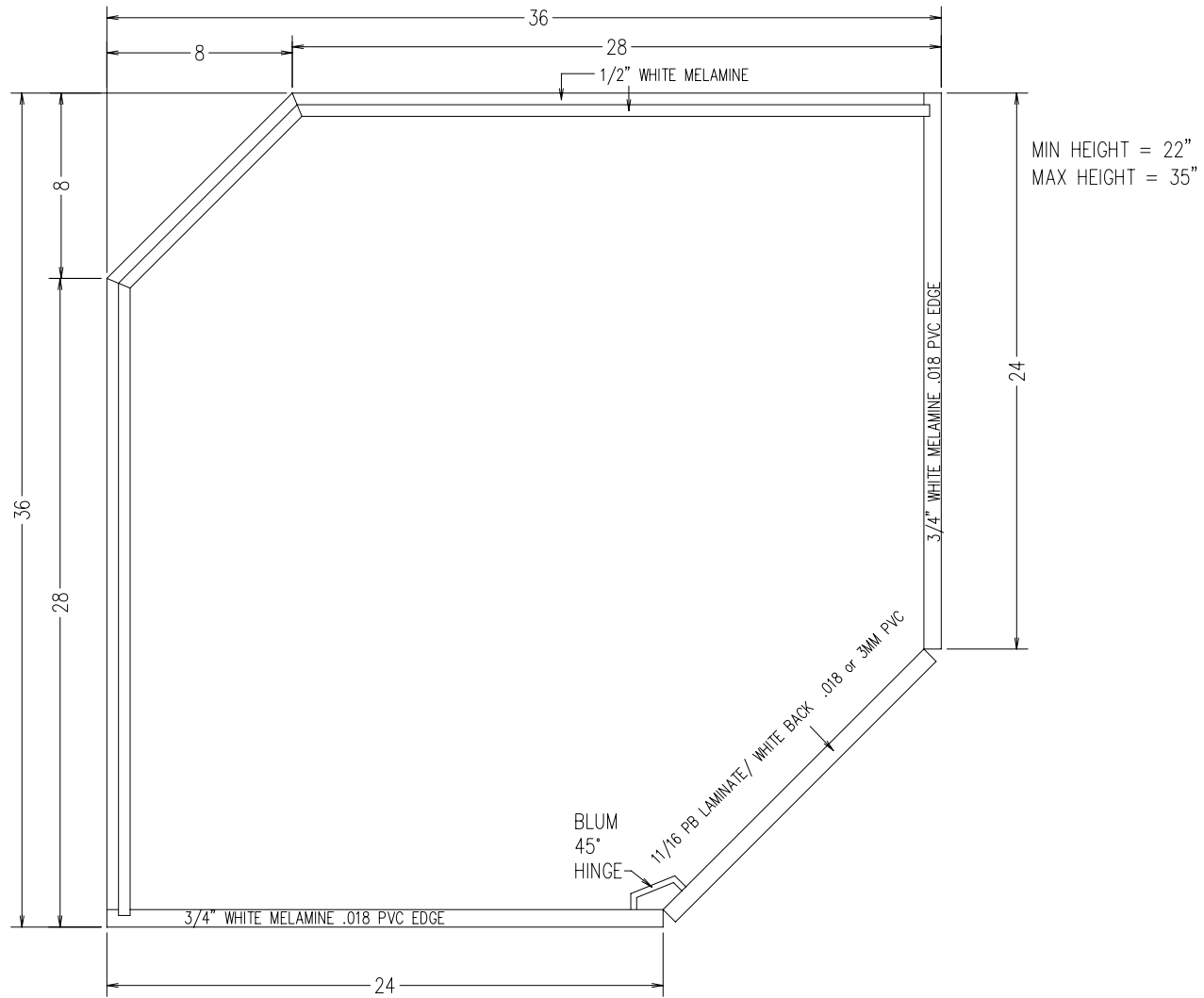
TYPICAL B1D-CORNER
