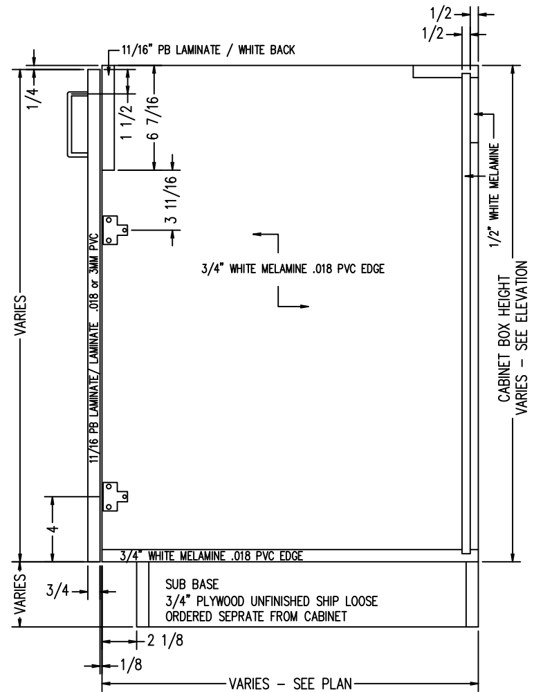
TYPICAL B2DSINK FOR SUB BASE
