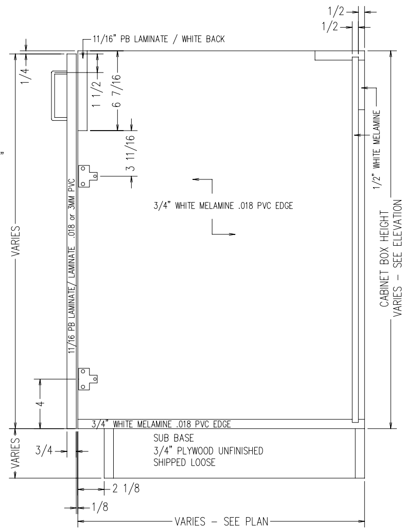
TYPICAL B2DSINK FOR SUB BASE SCALE: 1-1/2" = 1'-0"
