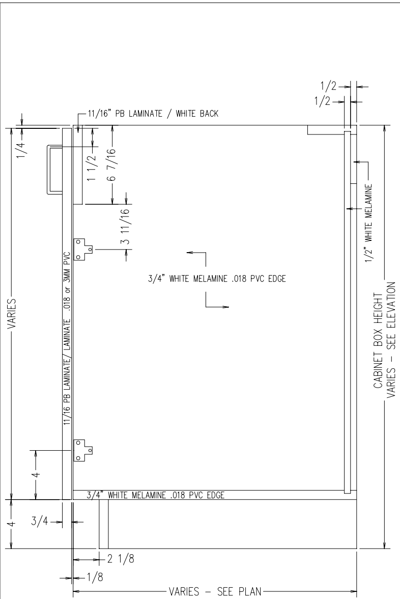
TYPICAL B2DSINK INTEGRAL TOE KICK SCALE: 1-1/2" = 1'-0"
