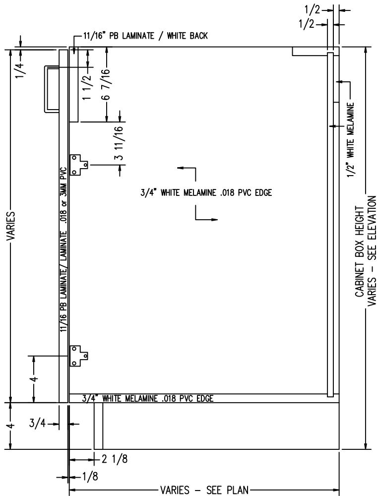
TYPICAL B2DSINK INTEGRAL TOE KICK
