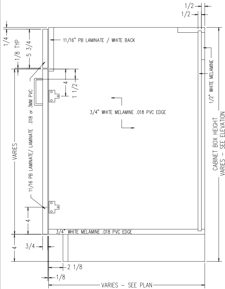
TYPICAL B2D1F INTEGRAL TOE KICK SCALE: 1-1/2" = 1'-0"
