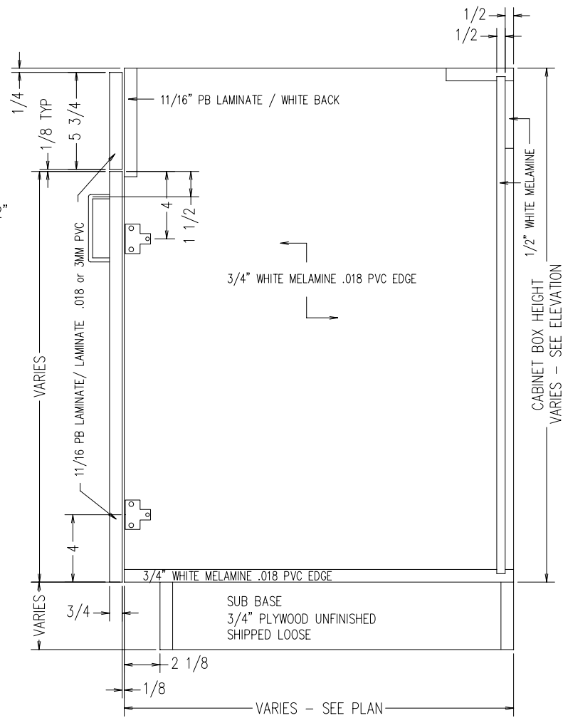
TYPICAL B2D1F FOR SUB BASE SCALE: 1-1/2" = 1'-0"
