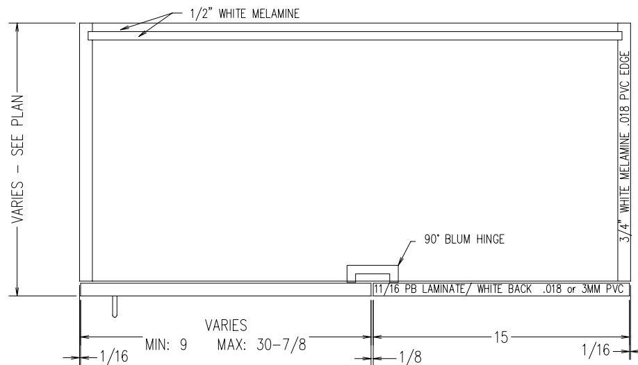
TYPICAL W1D-BLINDR TYPICAL W1D-BLINDL (OPPOSITE HAND) SCALE: 1-1/2" = 1'-0"
